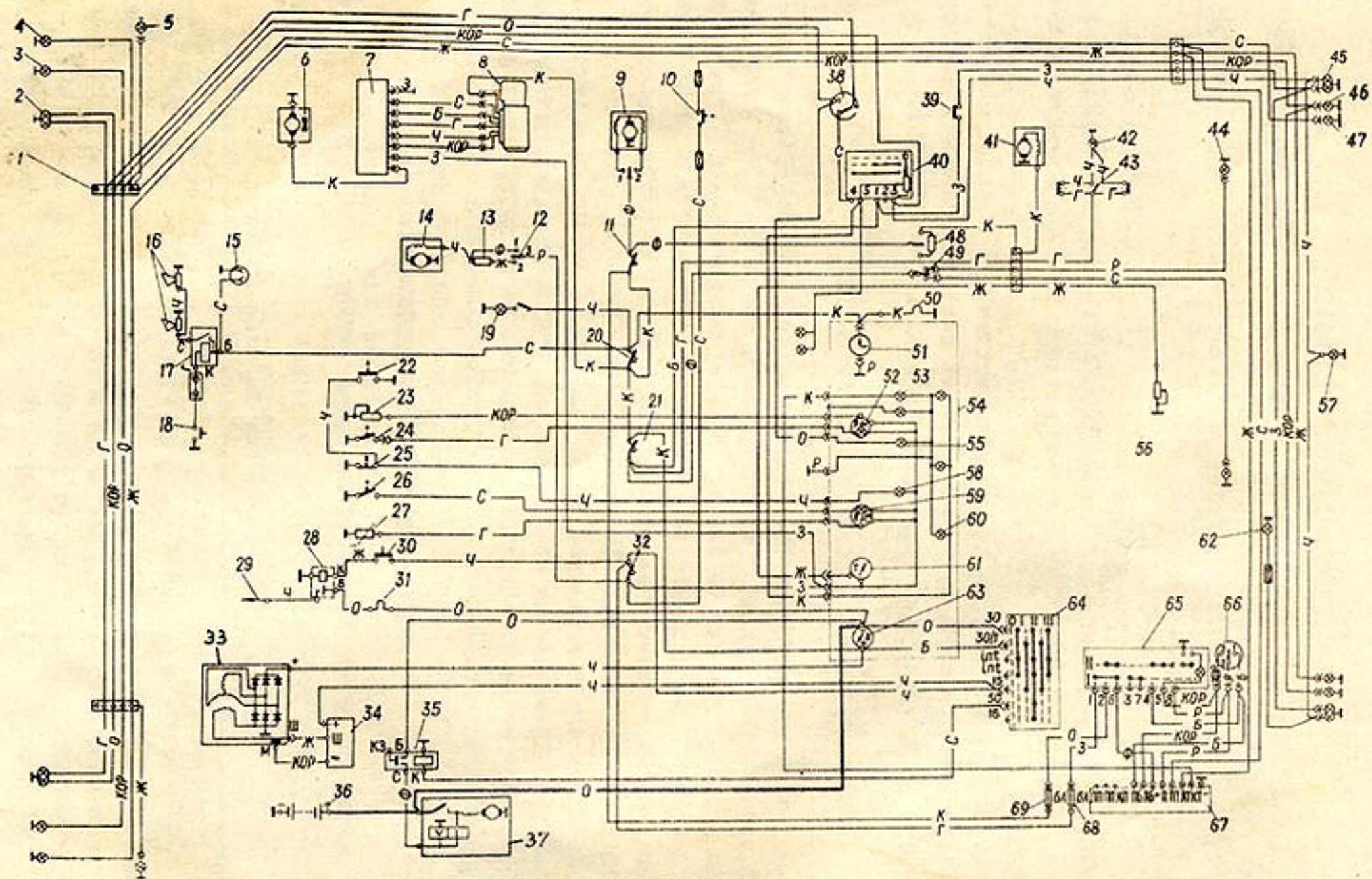
Fig.3. GAZ-24-56 Car Electric Equipment
